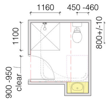
Figure 10 (f) Bathroom Design Option 6
